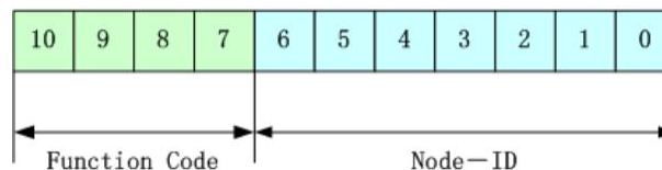
Figure 9-2 Default ID description diagram
