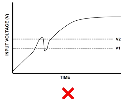
Figure 3-13 Non-monotonic power supply
