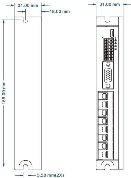
Hole position for fixation (孔位固定尺寸)
